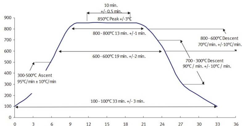
Typical 30 Minute Furnace Profile
